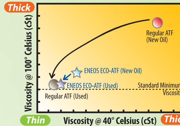
ENEOS ECO-ATF has minimal viscosity change after prolonged use
